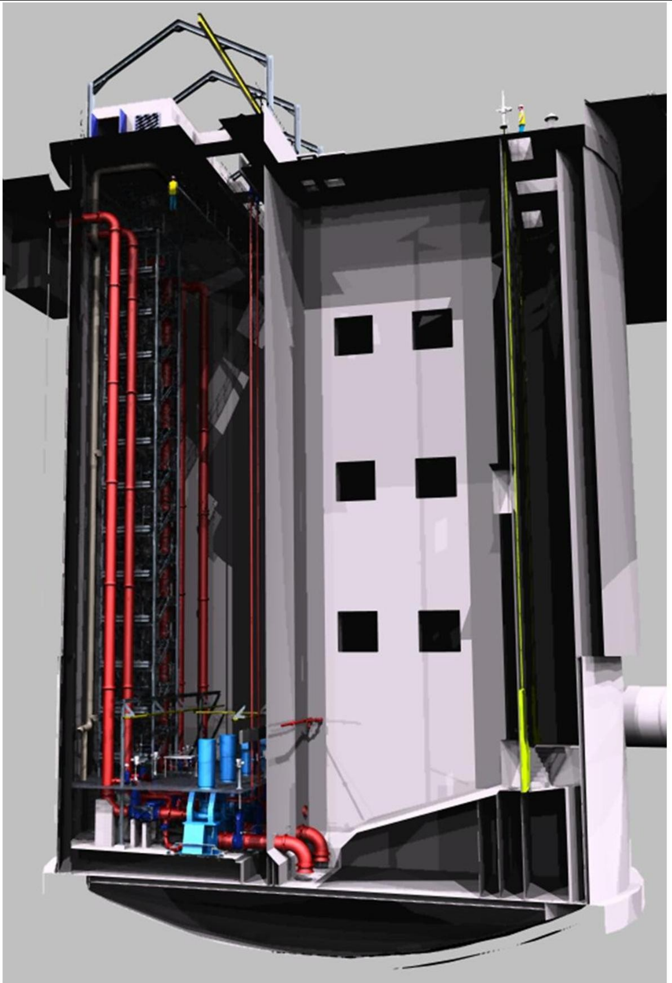
Photograph: An extract from the tender 3D model showing a section through the Terminal Pumping station.
